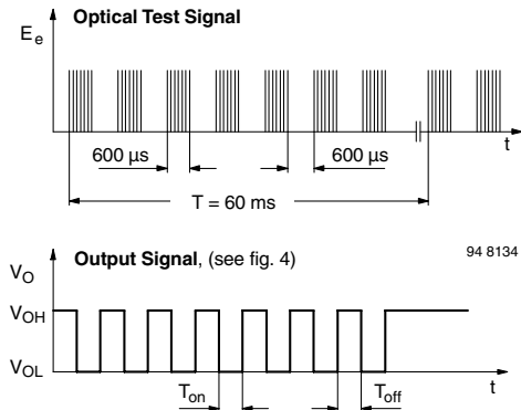
Figure 3. Output Function
